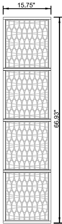
FRONT VIEW
